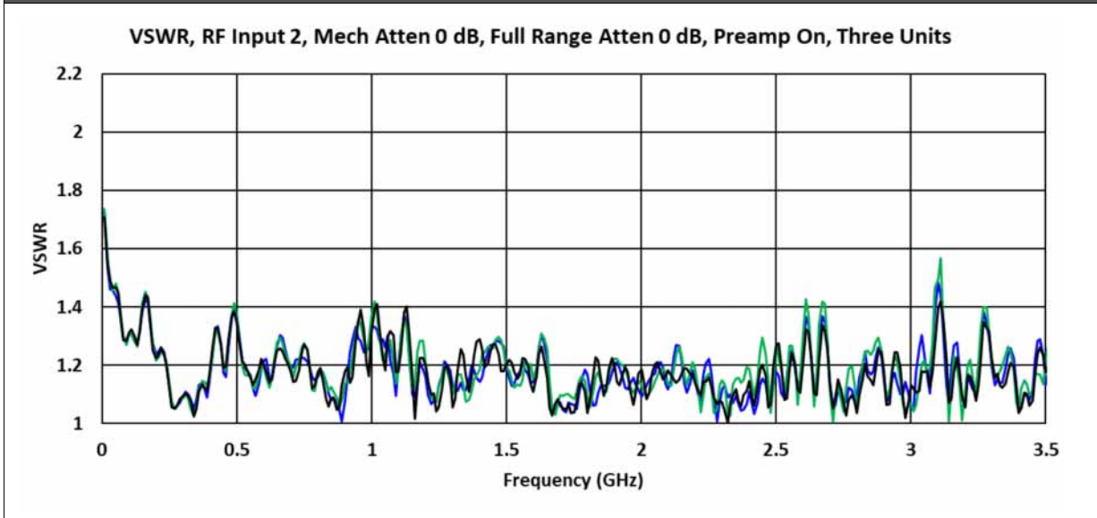
Nominal VSWR - Input 2 - Preamp On Band [Plot]
