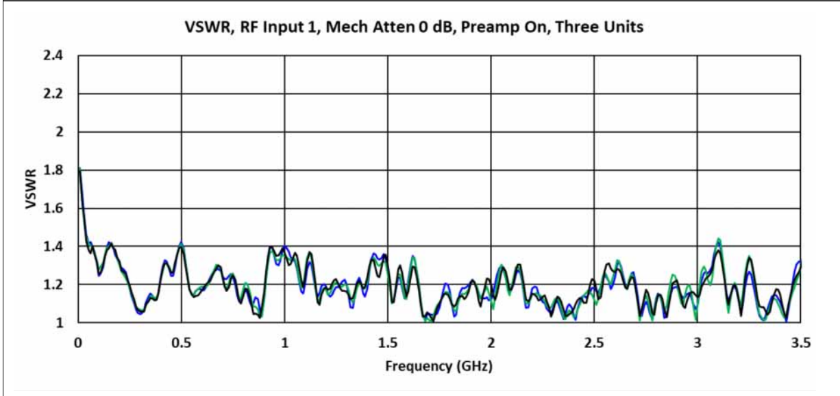
Nominal VSWR - Input 1 - Preamp On Band [Plot]
