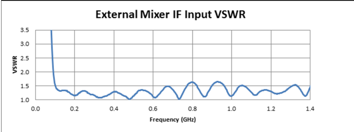
External Mixer IF Input VSWR [Plot]
